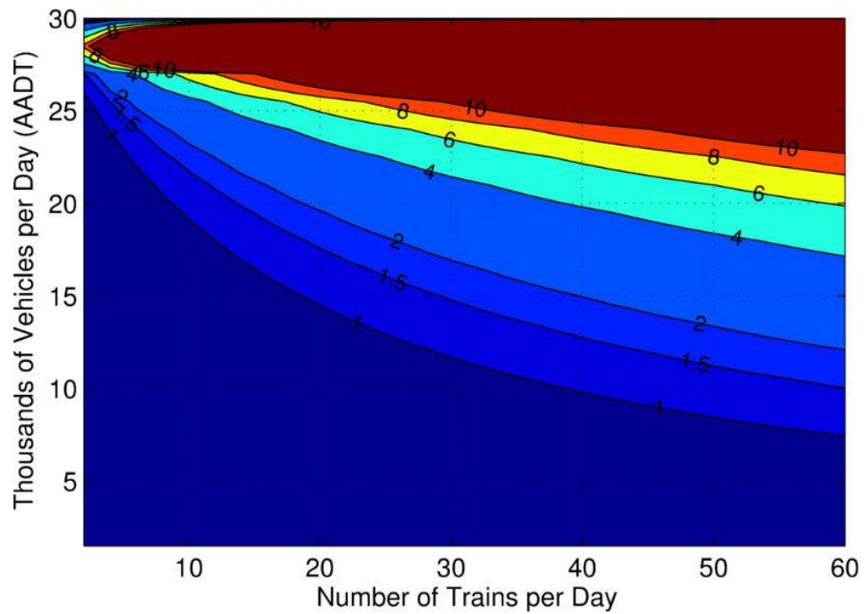
Figure 8.7 BCR for $5M Grade Separation Project @ 7% Discounting
