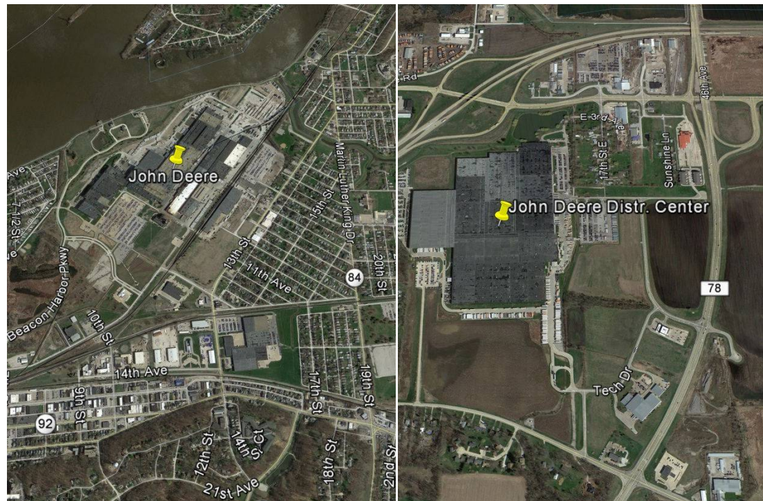
Figure 2.6 Transportation Equipment Cluster
